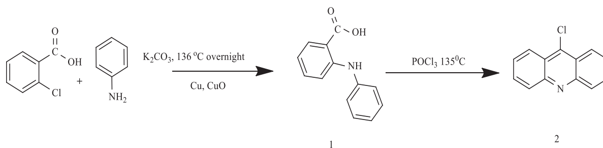
Scheme (1). Synthesis of 9-chloroacridine (2)
